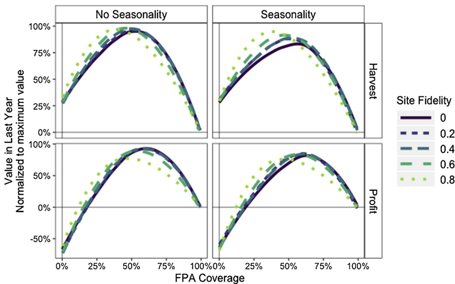
Fig. 2. Generalized model results for a multi-species indiscriminate lake fishery system. Harvest and profit in year 20 are shown under different FPA coverage sizes. Results are shown both with seasonality, which includes high- and low-water periods, and without seasonality. Lines are color coded based on the species guilds' site fidelity. This number represents the fraction of fish that stay in their cell instead of moving to adjacent cells.
