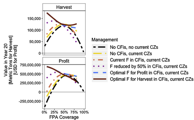
Fig. 4. Harvest and Profit in Tonle Sap in year 20 under different management scenarios and FPA coverage sizes. The FPA coverages include the current conservation zones (CZ) as well as additional randomly placed FPAs to achieve a certain coverage percentage. Line colors correspond to different management scenarios. (For interpretation of the references to colour in the text, the reader is referred to the web version of this article.)
